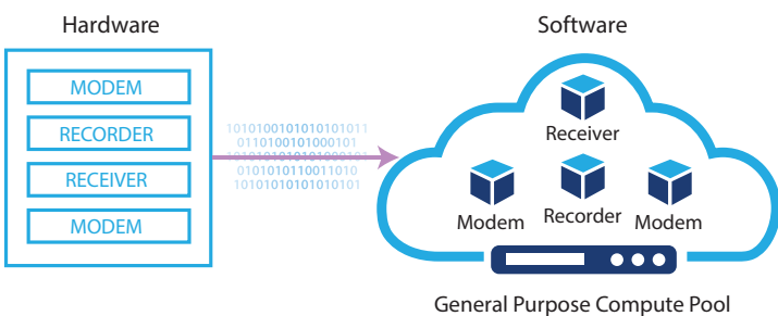
Virtualization in satellite ground systems includes the transition from proprietary hardware to software that performs the necessary functions virtually on general purpose computers.
